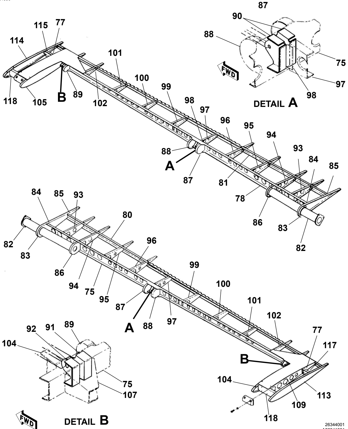
ELEVATOR INSTALLATION Figure 01. (Sheet 2)
