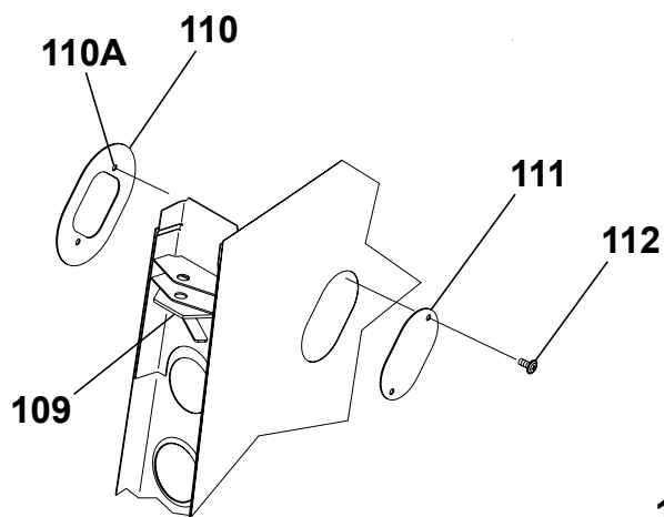
DETAIL D
