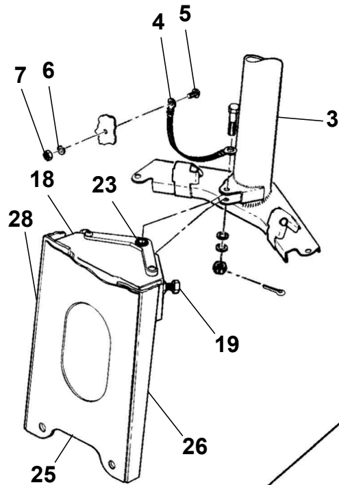
DETAIL D
