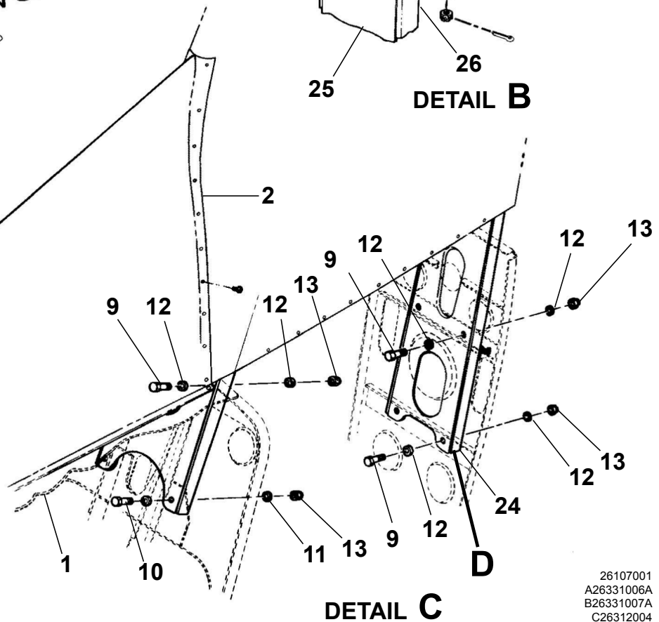
VERTICAL FIN INSTALLATION Figure 04. (Sheet 1)
