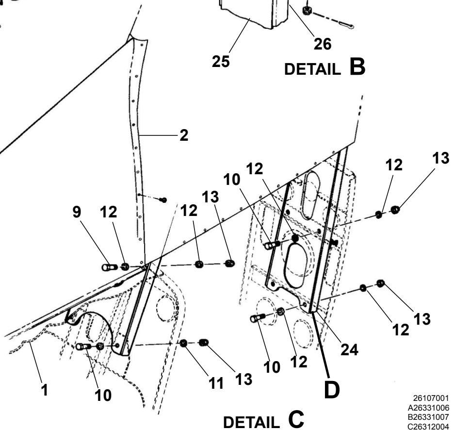
VERTICAL FIN INSTALLATION Figure 03. (Sheet 1)
