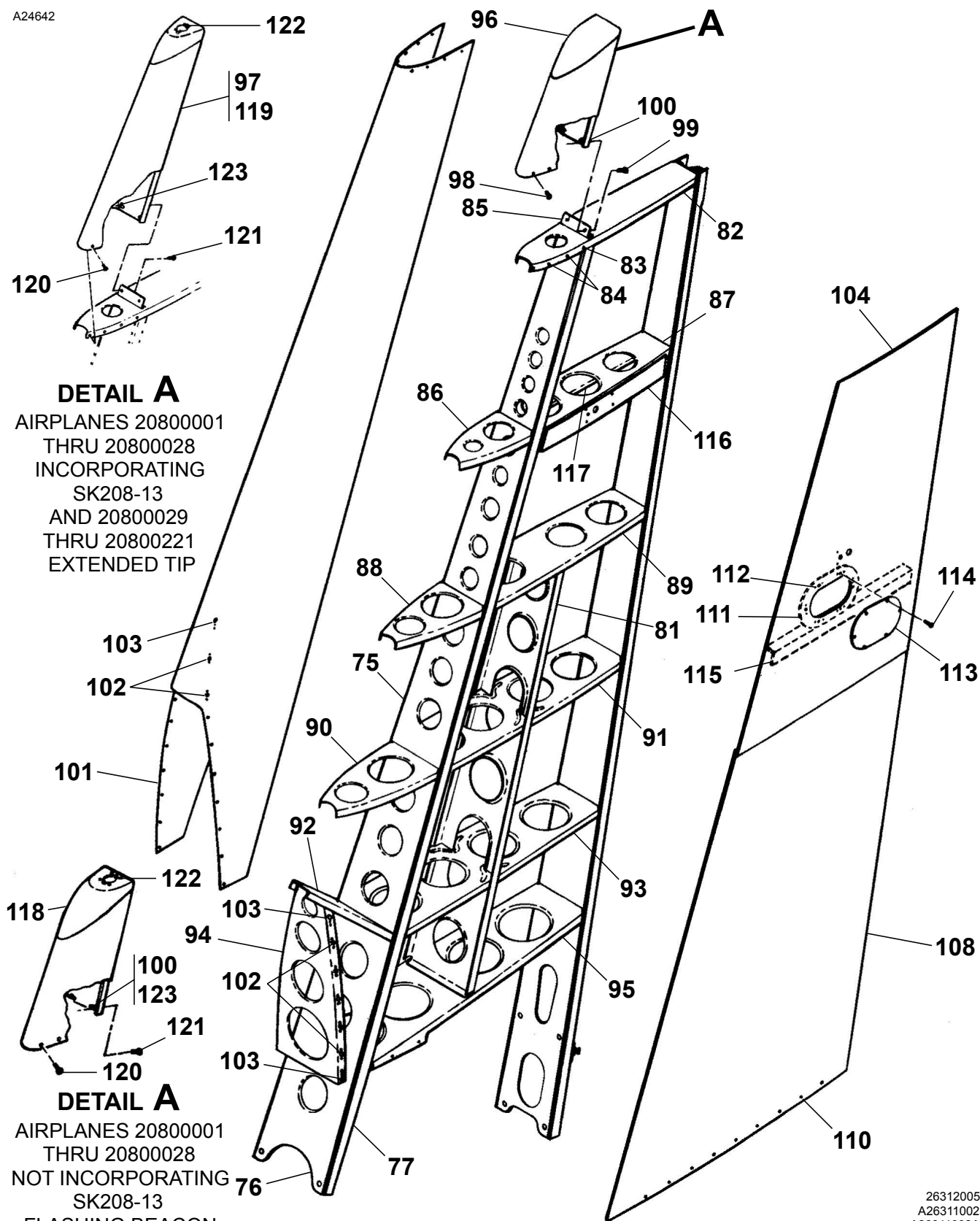
VERTICAL FIN INSTALLATION Figure 01. (Sheet 2)
