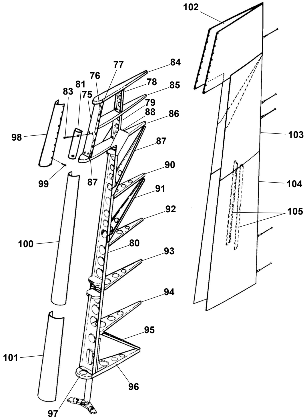
RUDDER INSTALLATION - 208B Figure 04. (Sheet 2)
