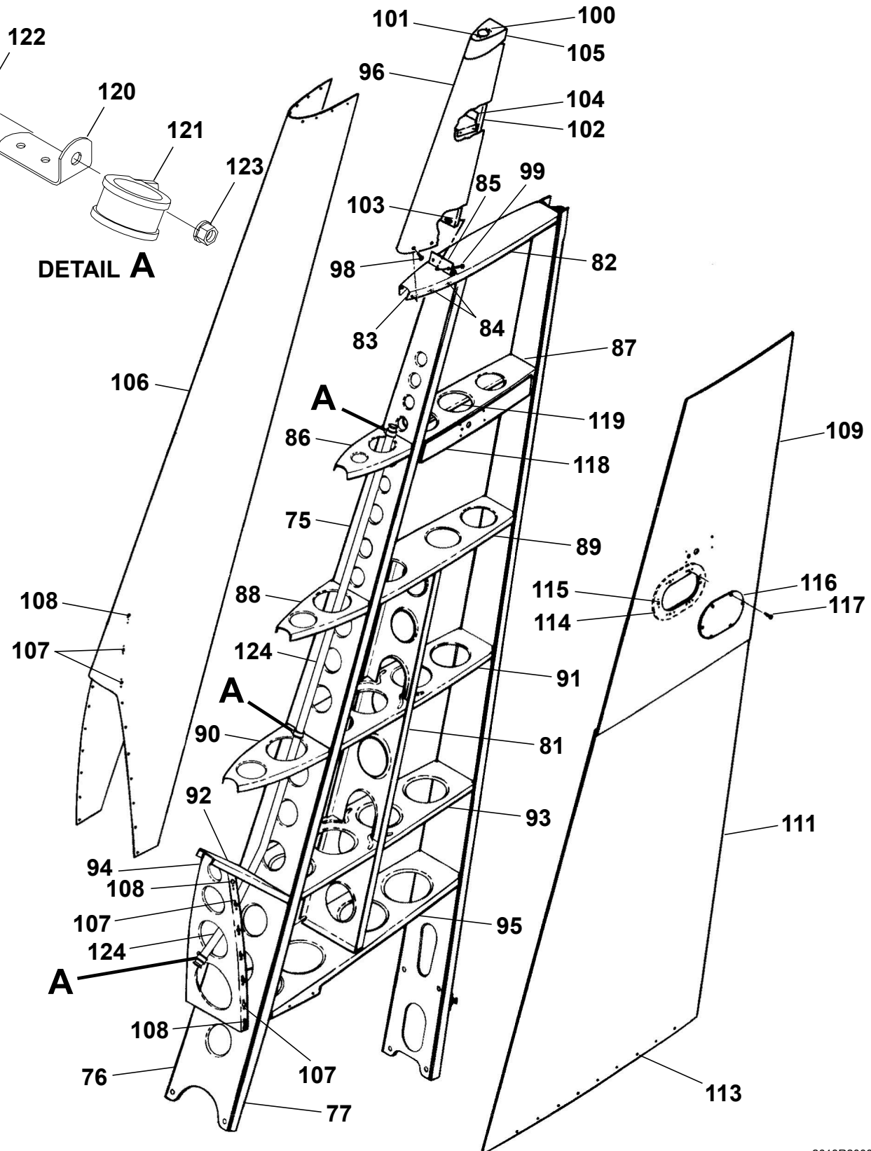
VERTICAL FIN INSTALLATION Figure 04. (Sheet 2)
