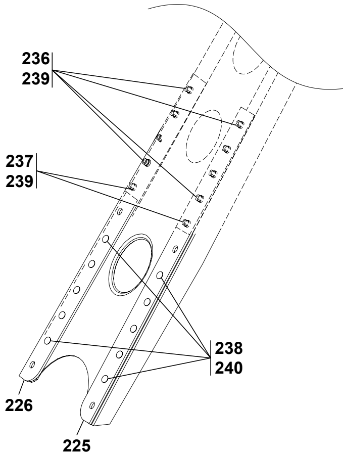
DETAIL B
