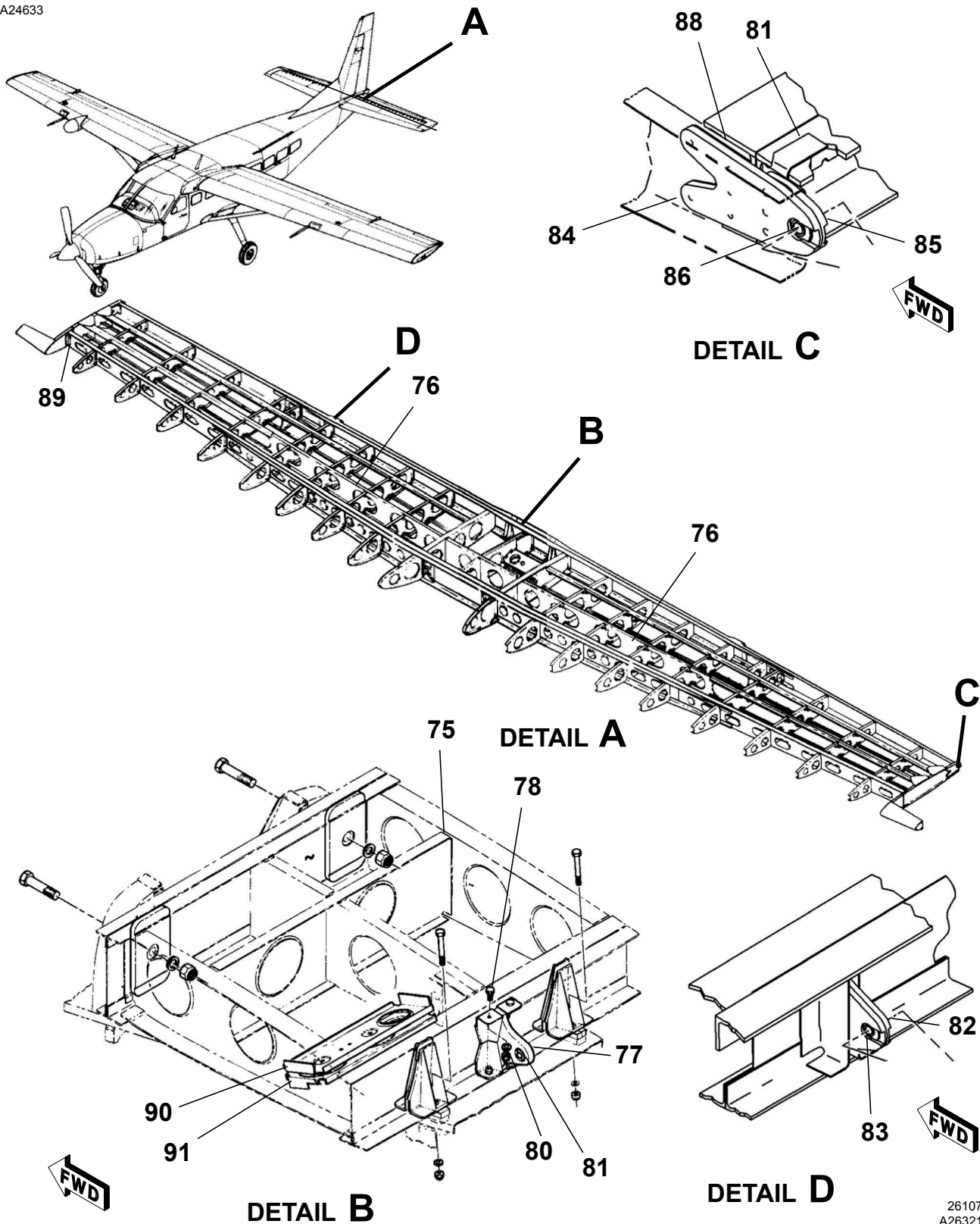
HORIZONTAL STABILIZER INSTALLATION Figure 02. (Sheet 2)
