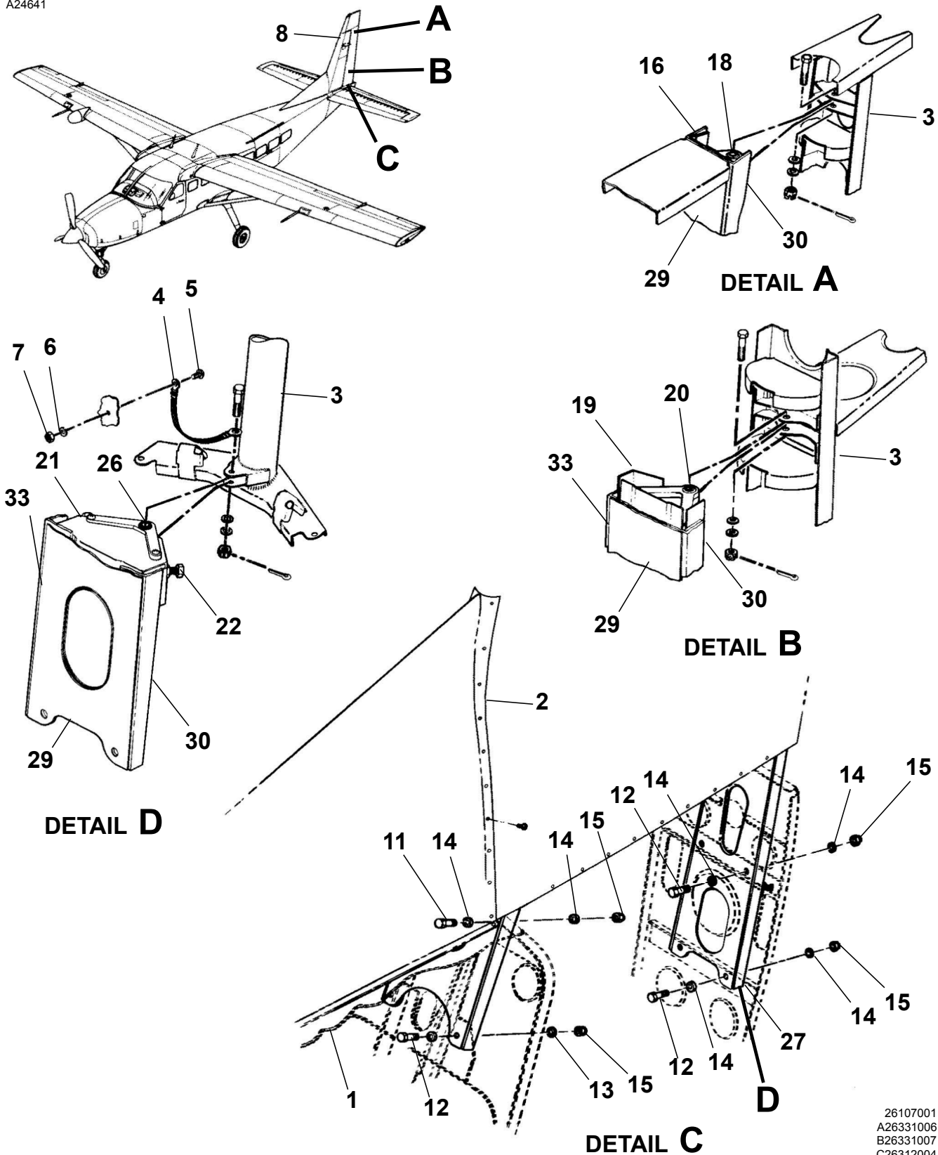
VERTICAL FIN INSTALLATION Figure 01. (Sheet 1)
