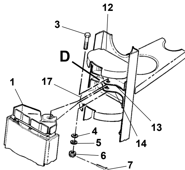
DETAIL B
