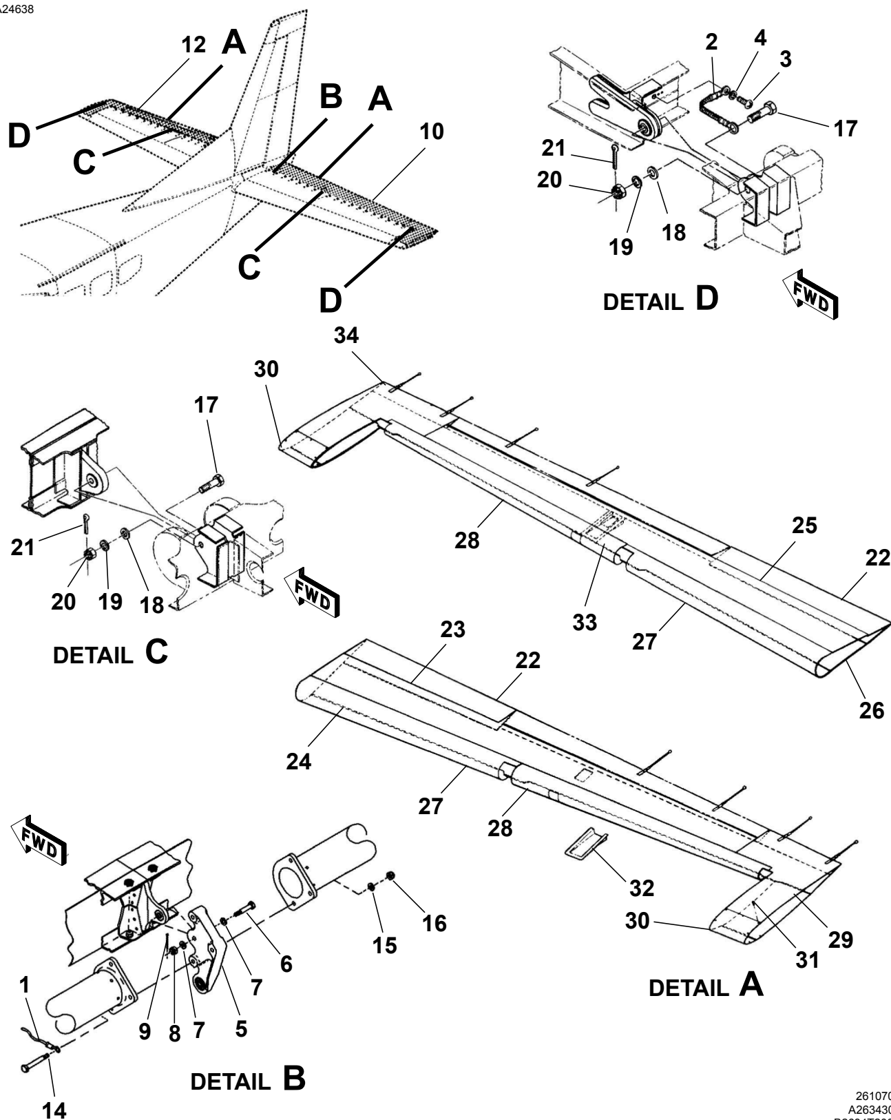
ELEVATOR INSTALLATION Figure 02. (Sheet 1)
