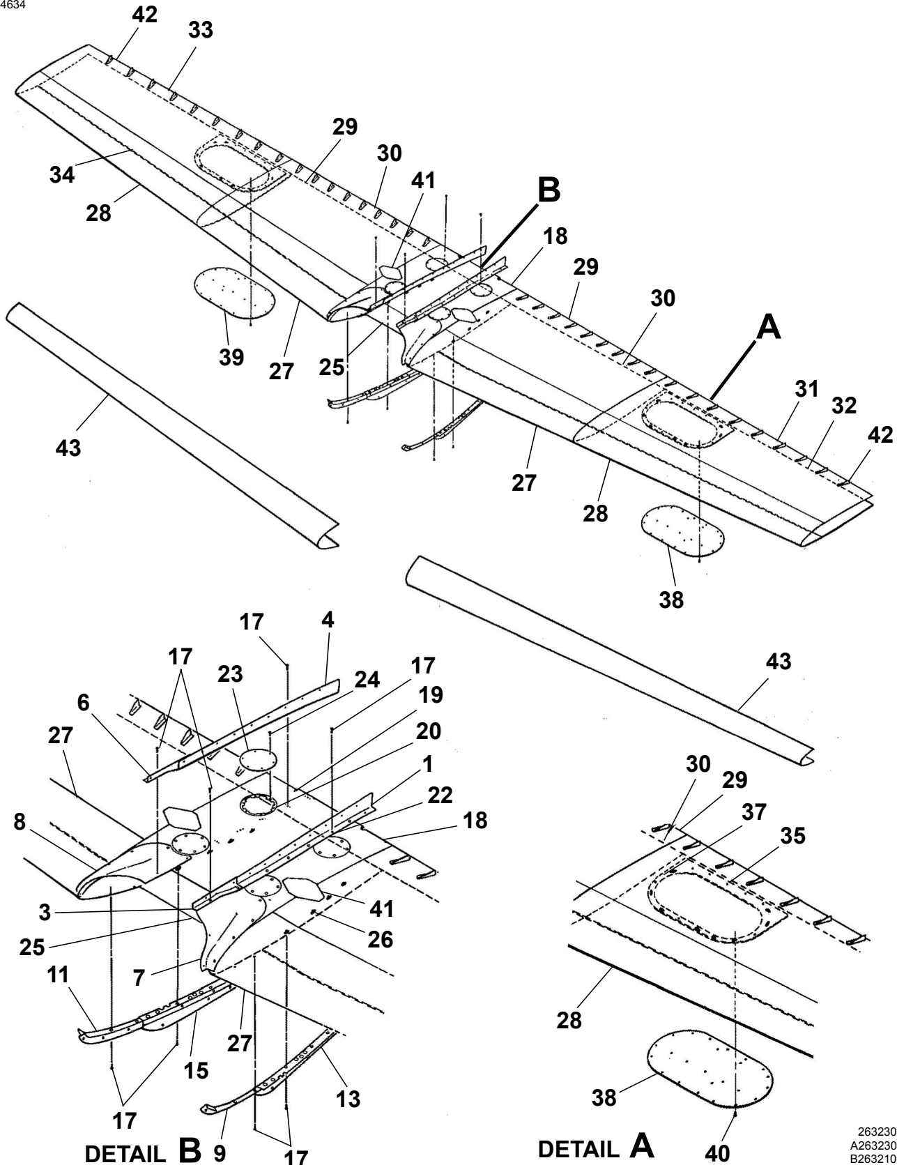
STABILIZER SKINS AND FAIRINGS Figure 01. (Sheet 1)
