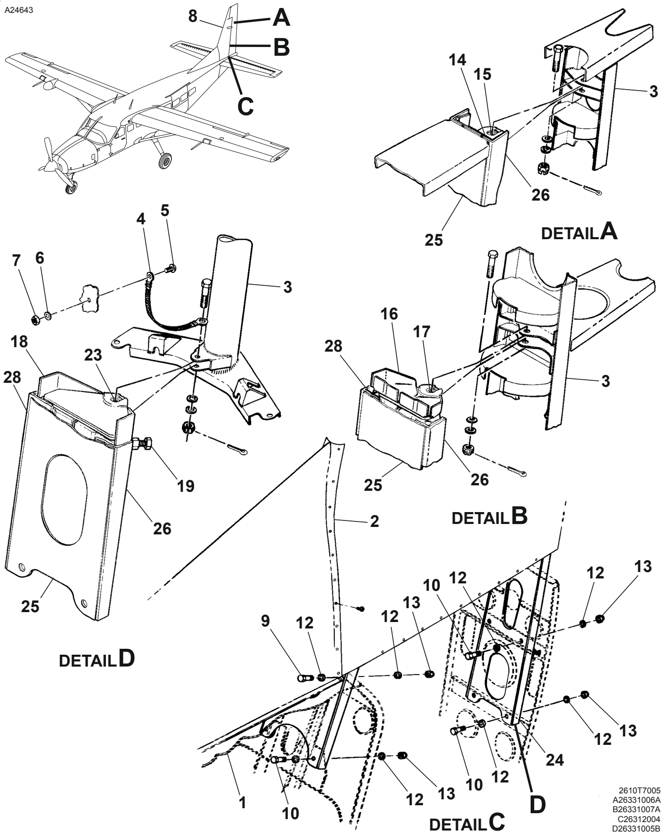
VERTICAL FIN INSTALLATION Figure 02. (Sheet 1)
